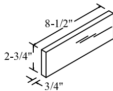
OVERSIZE THIN CORNER TC-000
