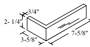
MODULAR THIN CORNER TC-020
